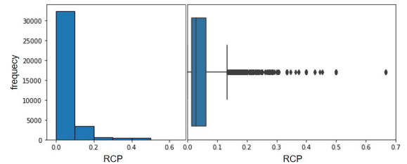
Figure 3: Distribution of Repeat Customer Probability.
